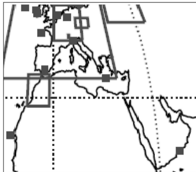
Little Ice Age (1300-1900 A.D.)
