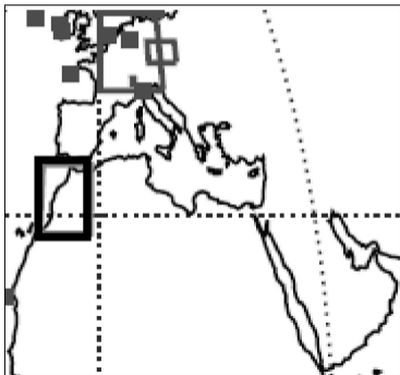
Medieval Warm Period (800-1300 A.D.)
